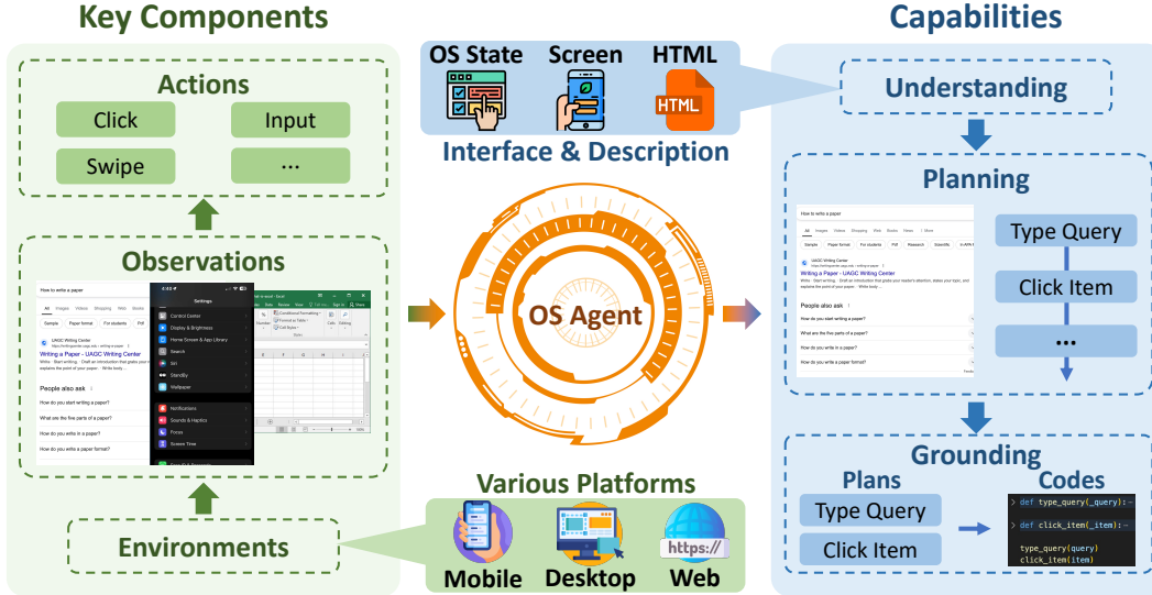
Figure 2: Fundamentals of OS Agents.
